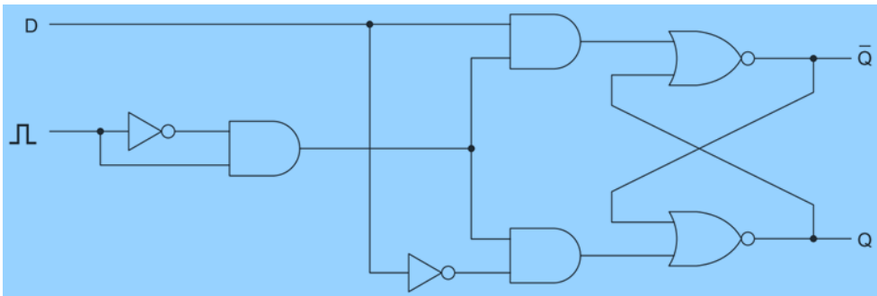
5-nji çyzgy. D -trigger
